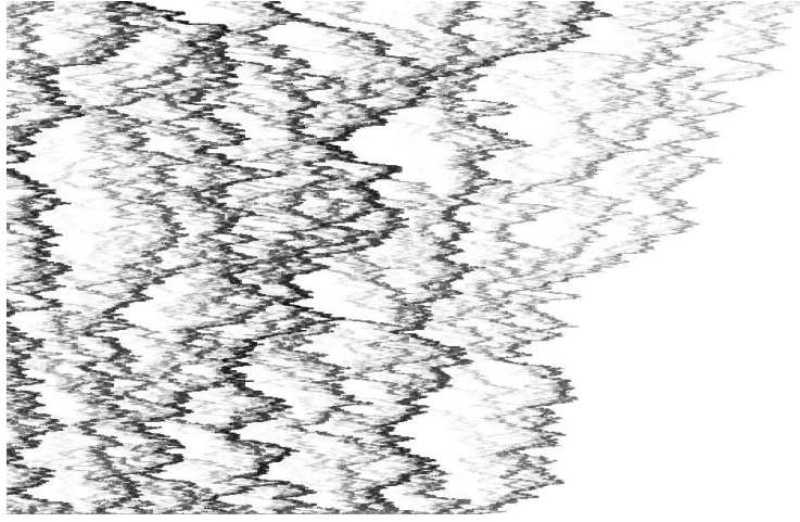
Figure 5: Example of an asymmetric flow: the one-sided erosion flow with \beta = 0 and \nu = \delta_1 . This flow has left and right speeds \beta_- = -\infty and \beta_+ = 2 , respectively. The picture shows a rectangle of 3.2 units of space (horizontal) by 0.4 units of time (vertical). The initial state is Lebesgue measure up to the point 1.9 and zero from there onwards.
