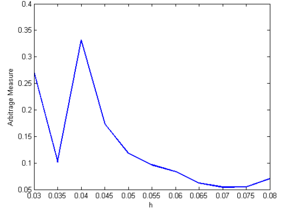
Fig. 2b: Arbitrage measure for DAX options IV surface
