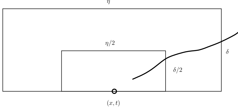
Figure 14: A path causing the event A_{\delta, \eta}(x, t) to occur.
