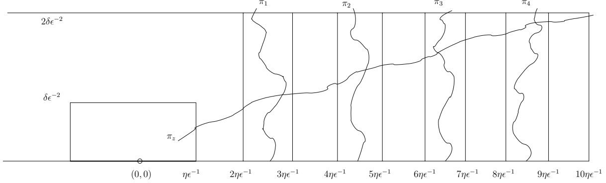
Figure 15: The random walks \pi_1, \pi_2, \pi_3, \pi_4 start respectively at 2.5\eta\epsilon^{-1} , 4.5\eta\epsilon^{-1} , 6.5\eta\epsilon^{-1} and 8.5\eta\epsilon^{-1} at time 0 and each stays within an interval of size \eta\epsilon^{-1} up to time 2\delta\epsilon^{-2} . The walk \pi_z starts from z inside the rectangle [-\eta\epsilon^{-1}, \eta\epsilon^{-1}] \times [0, \delta\epsilon^{-2}] and crosses the right side of the rectangle [-10\eta\epsilon^{-1}, 10\eta\epsilon^{-1}] \times [0, 2\delta\epsilon^{-2}] before time 2\delta\epsilon^{-2} without meeting (\pi_i)_{1 \leq i \leq 4} .
