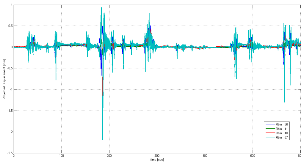
Figure 7 – Vertical deflections of points No. 1, 2, 6 and 3 during 10min measurement
