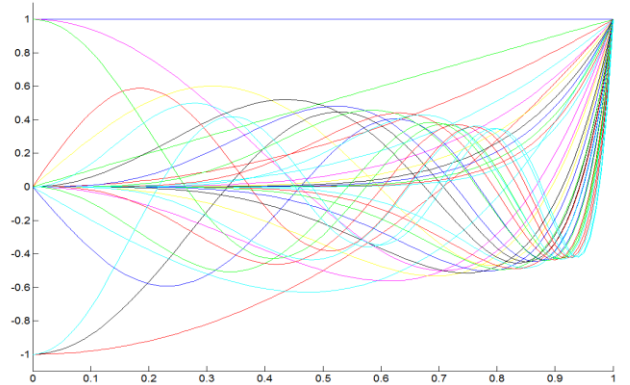
Fig. 2 Zernike Polynomials up to 10th degree
