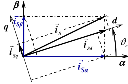
Fig. 4. 2D \alpha - \beta and d - q coordinate systems
