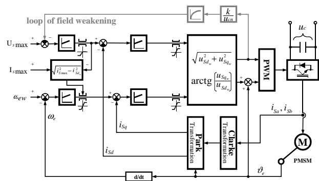
Fig. 6. Speed control of PMSM with field weakening loop.
