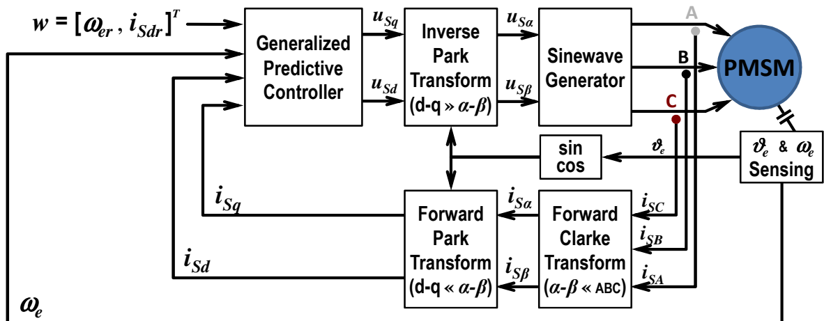
Fig. 7. Speed control of PMSM by Generalized Predictive Control
