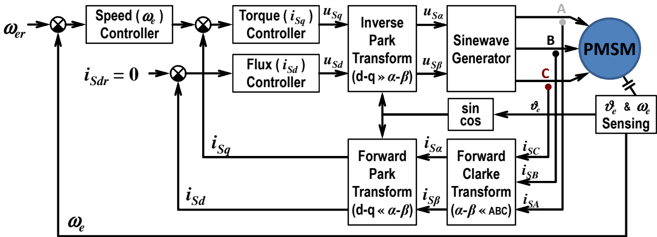
Fig. 5. Speed control of PMSM by vector control (two-step cascade control)
