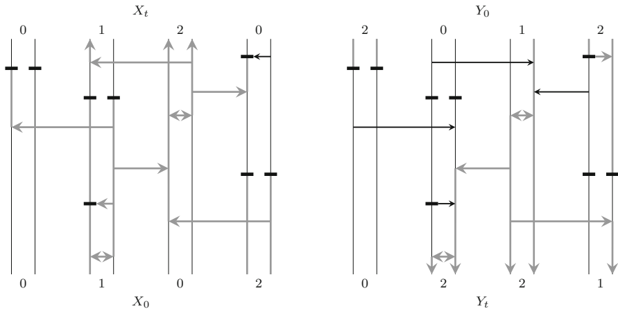
Fig. 2 Graphical representation of a two-stage contact process and its dual
