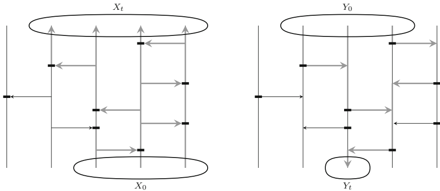
Fig. 1 Graphical representation of a voter model and its dual
