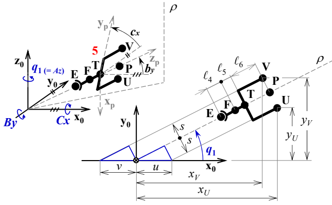
Fig. 5. Detail of the link 5 representing the robot gripper with stroke s .
