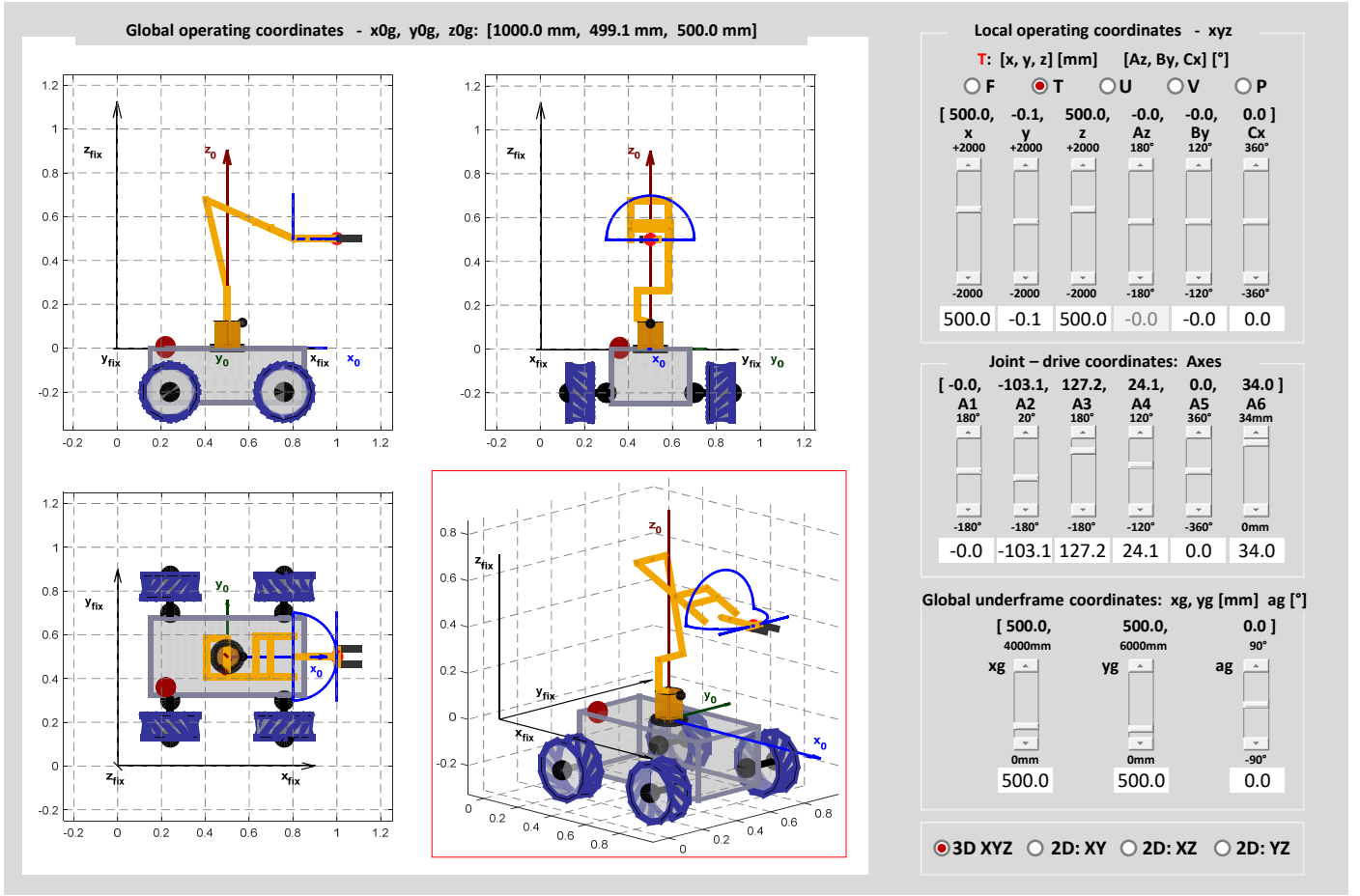
Fig. 2. Basic views: front, top plan, side and 3D view with definitions of global coordinate system ( x_{fix}, y_{fix}, z_{fix} ) and local coordinate system ( x_0, y_0, z_0 ).
