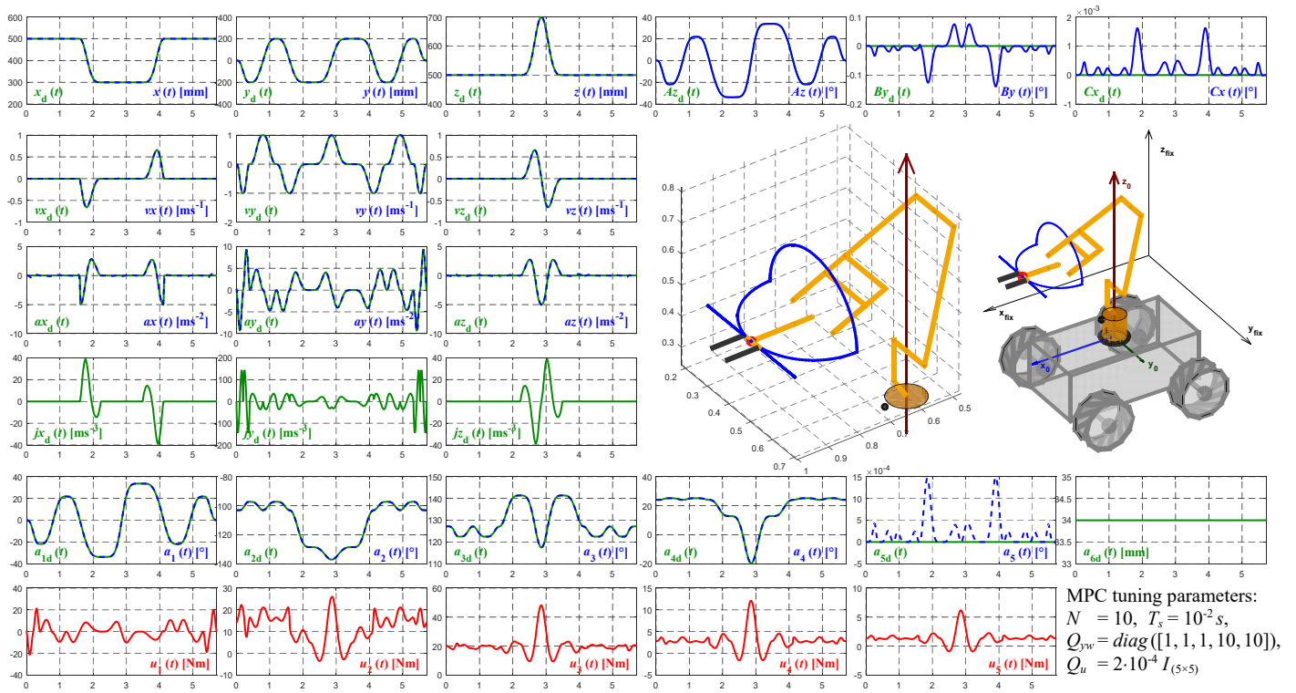
Fig. 6. Time histories of kinematic quantities and control actions presenting in local motion control of 5 DOF articulated robot arm including used MPC parameters.
