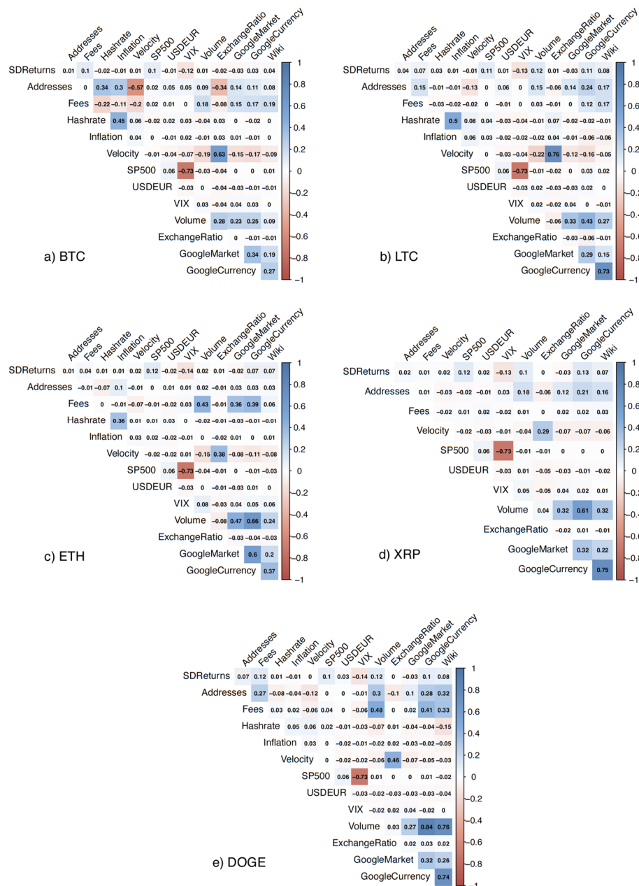
Fig. 3 Correlation matrices of the datasets. Note: The color gradually changes from dark blue ( \rho = 1 ) through white ( \rho = 0 ) to dark red ( \rho = -1 ) as the Pearson correlation coefficient \rho decreases; see the specific range of colors on the right side of the figures. “SDReturns” represents r_t/\hat{\sigma}_t . Based on N = 2221 observations and rounded to two decimal digits
