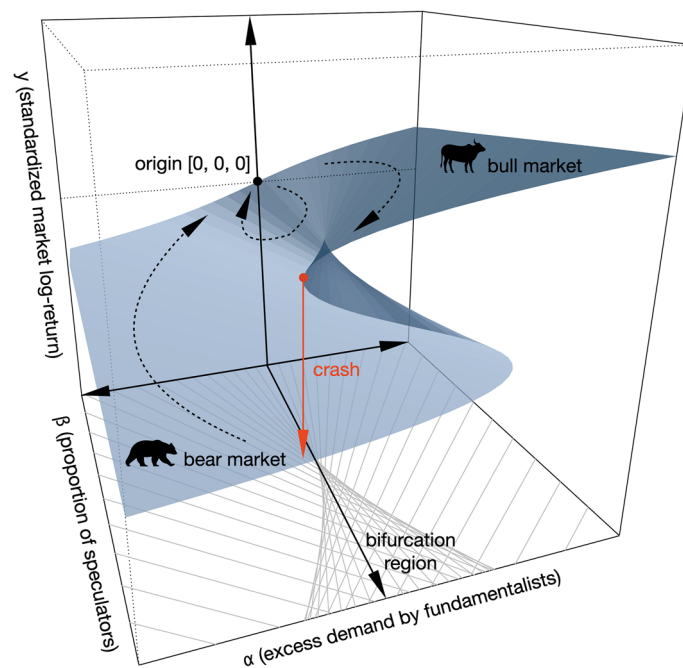
Fig. 1 An illustrative equilibrium response surface of the cusp catastrophe model and the cyclical dynamics of the market. Source: produced in R using the cusp package version 2.3.3. and completed by the authors
