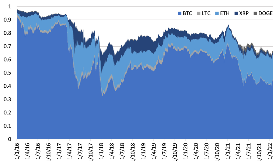
Fig. 2 Combined market capitalization of BTC, LTC, ETH, XRP, and DOGE. Note: Depicted in relation to the total cryptocurrency market capitalization between January 1, 2016, and January 31, 2022. Data are retrieved from coinmarketcap.com
